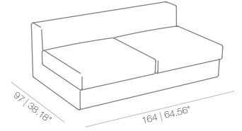
ELEMENT B3
